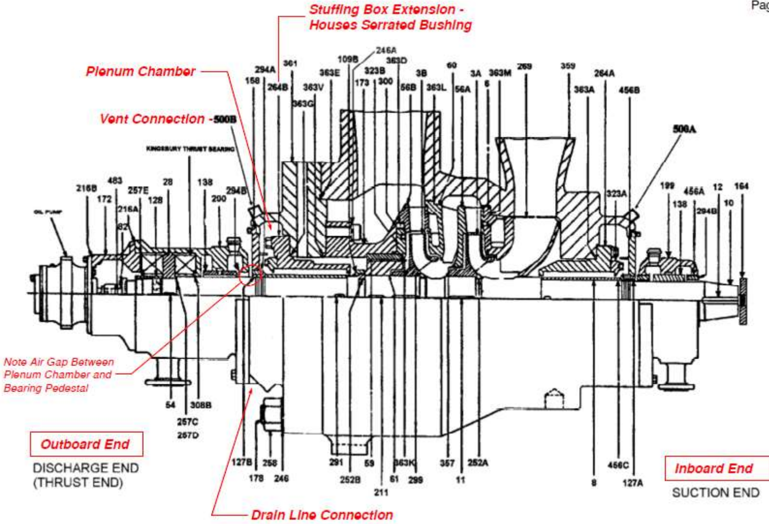
Main Feed Pump Diagram Ingersoll-Rand (Flowserve) 16X19-2CA
