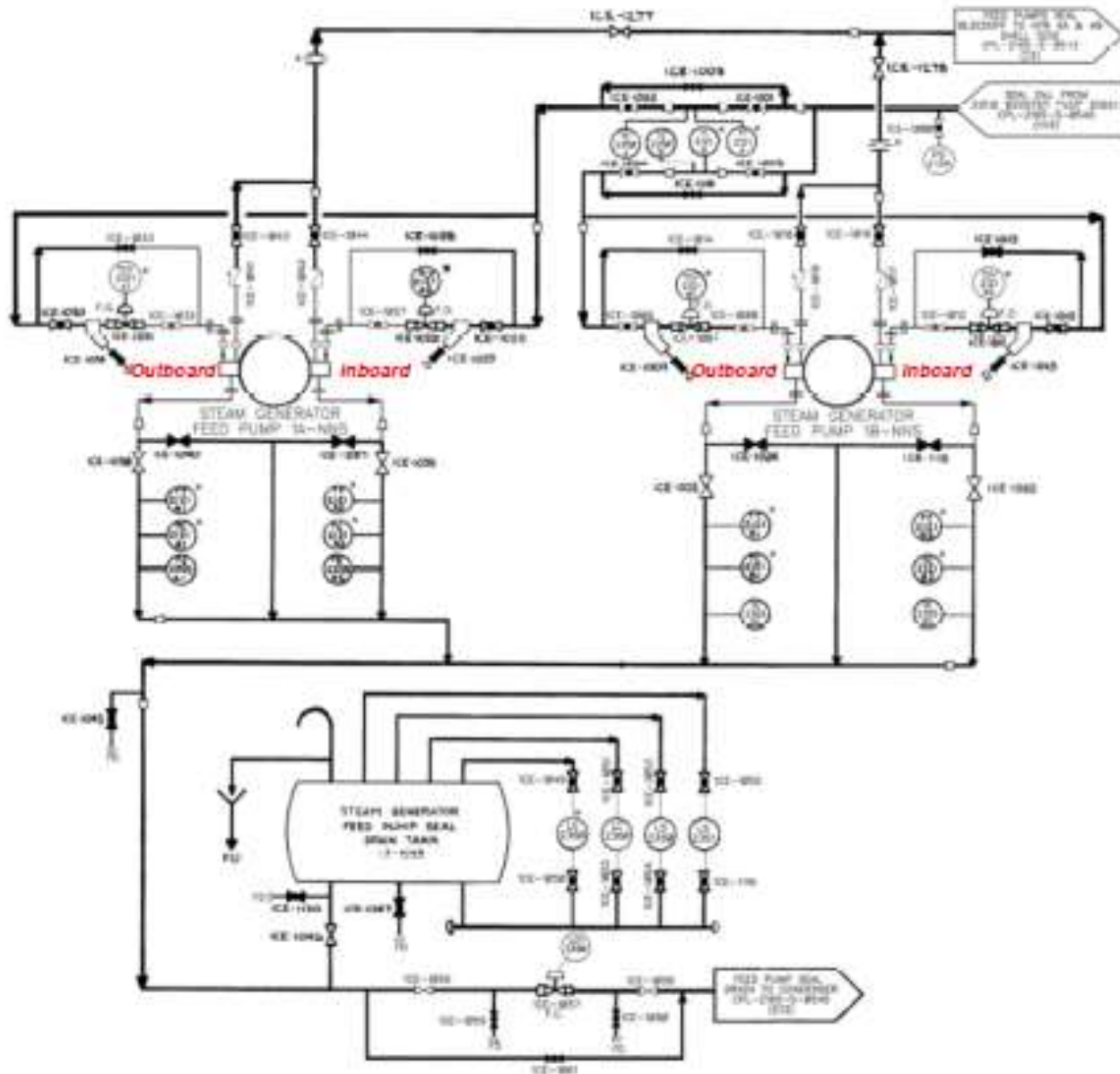
STEAM GENERATOR FEED PUMP SEAL WATER SYSTEM
